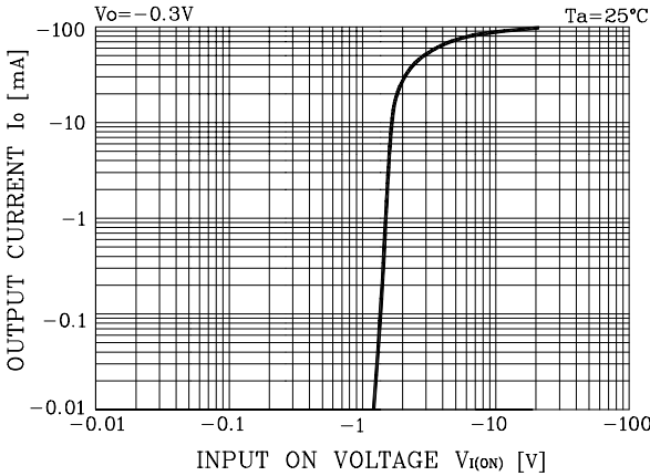
Fig. 1 I_o - V_{I(ON)}
